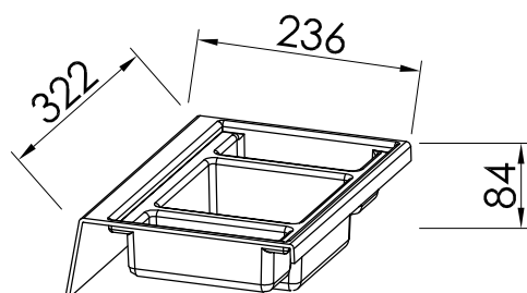
ORGANIZATOR PREDALA SPOD. 350 DRAWER ORGANIZER BOTTOM 350
