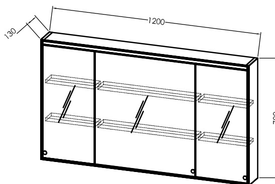
TO 120 BL - LED, SW, S
