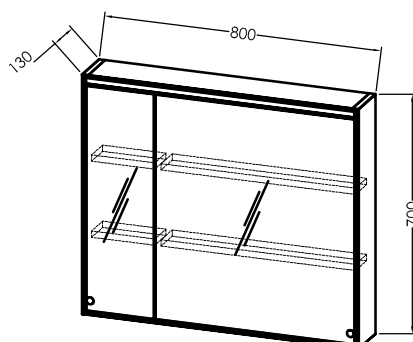
TO 80 BL - LED, SW, S
