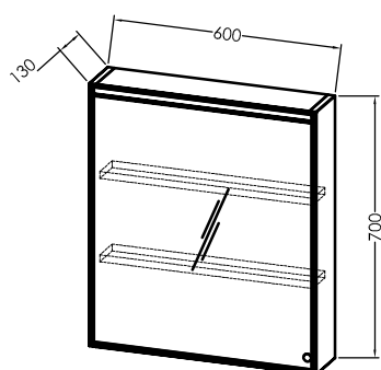
TO 60 BL - LED, SW, S
